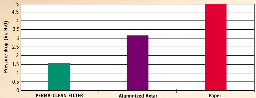
Average Pressure Drop vs Cartridge Type
