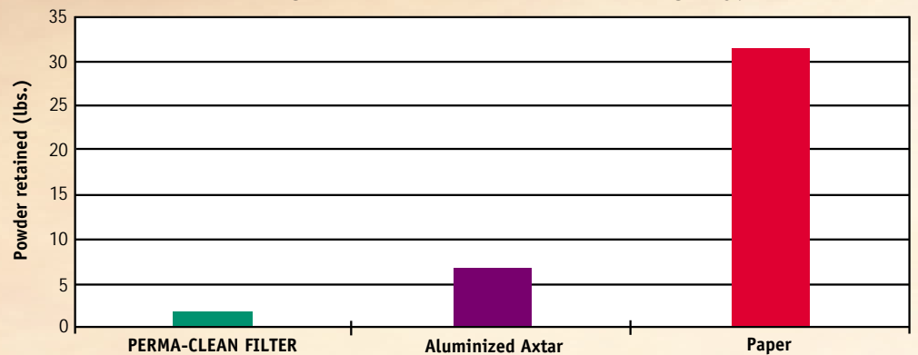
Average Powder Retained vs Cartridge Type
