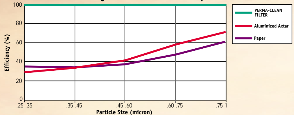
Media Efficiency vs Particle Size at 10 fpm
